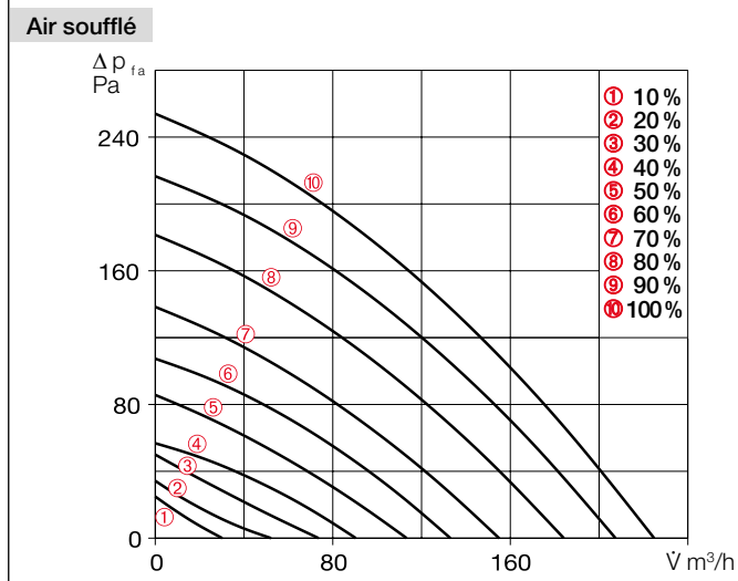
Characteristic curve KWL 200 W
